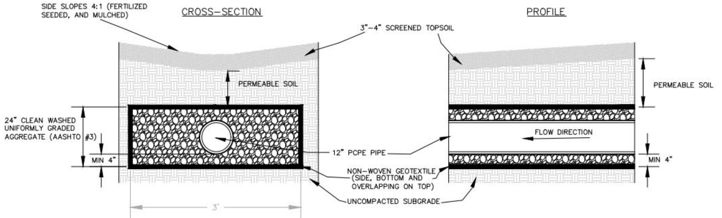
INFILTRATION SWALE CROSS-SECTION AND PROFILE DETAIL
